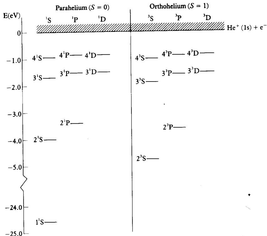
6.2 The experimental values of the lowest energy levels of helium. The energy scale is chosen so that E = 0 corresponds to the ionisation threshold. The configuration of each level is of the form 1s nl . The doubly excited states (for example 2s nl ) are at positive energies on this scale, within the \text{He}^+(1s) + e^- continuum.
